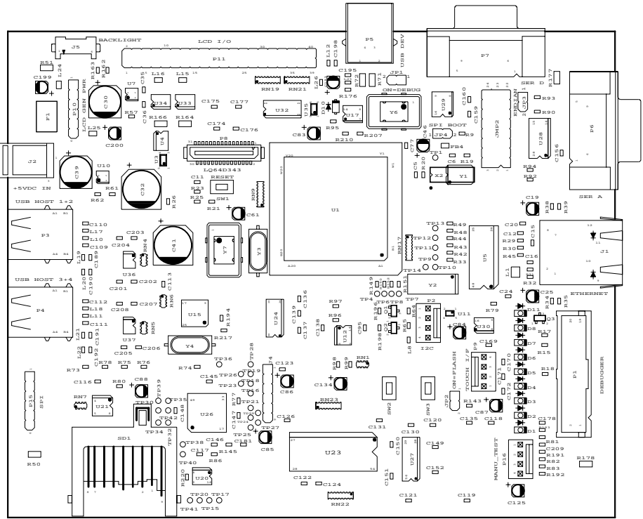
ASSEMBLY TOP (VIEWED FROM THE COMPONENT SIDE)
