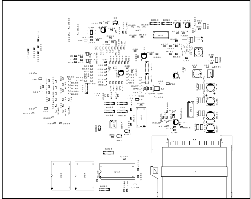
ASSEMBLY BOTTOM (MIRRORED - VIEWED FROM THE SOLDER SIDE)
