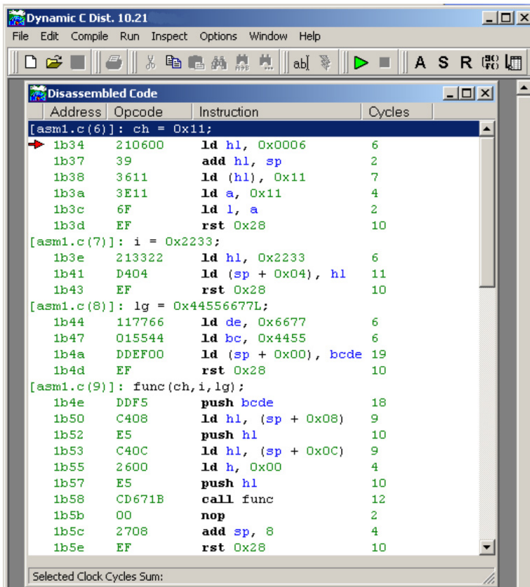
Figure 13.2 Disassembled Code Window
