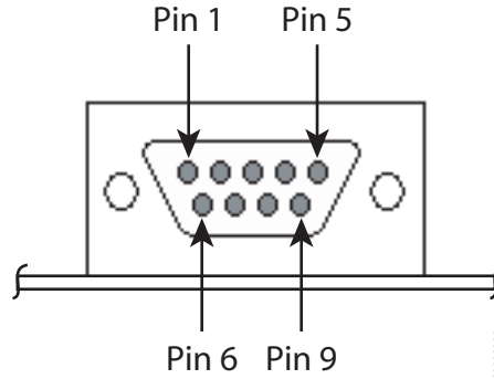
Primary Serial Port Pin Assignments
